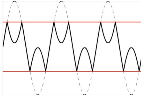
Figure 12.2. sine-wave distorted with folding
