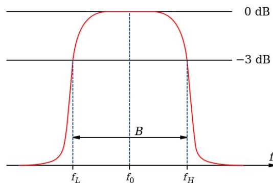
Figure 8.1. band-pass filter
