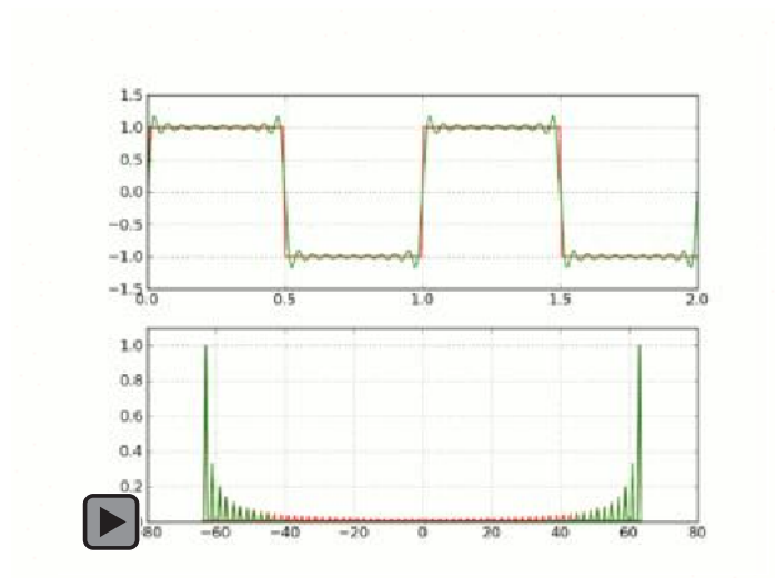
Figure 3.3. square wave
