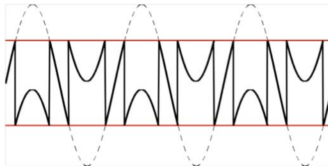
Figure 12.3. sine-wave distorted with wrapping
