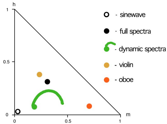
Figure 2.1. tristimulus diagram
