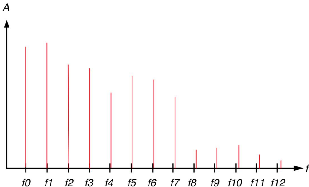
Figure 4.1. spectrum of nearly harmonic partials
