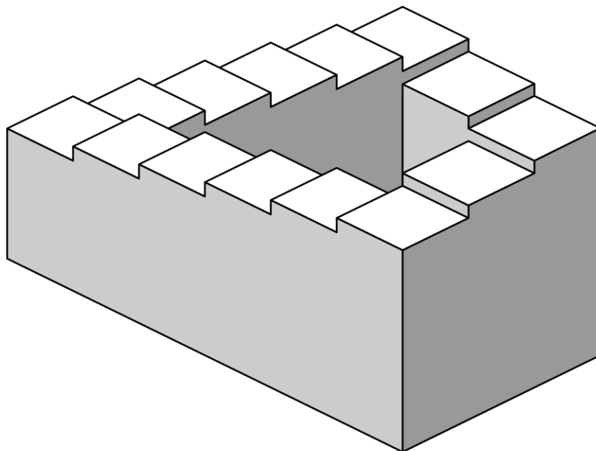
Figure 6.2. Penrose staircase
