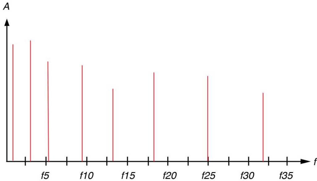
Figure 4.2. spectrum of widely spaced (parse) partials
