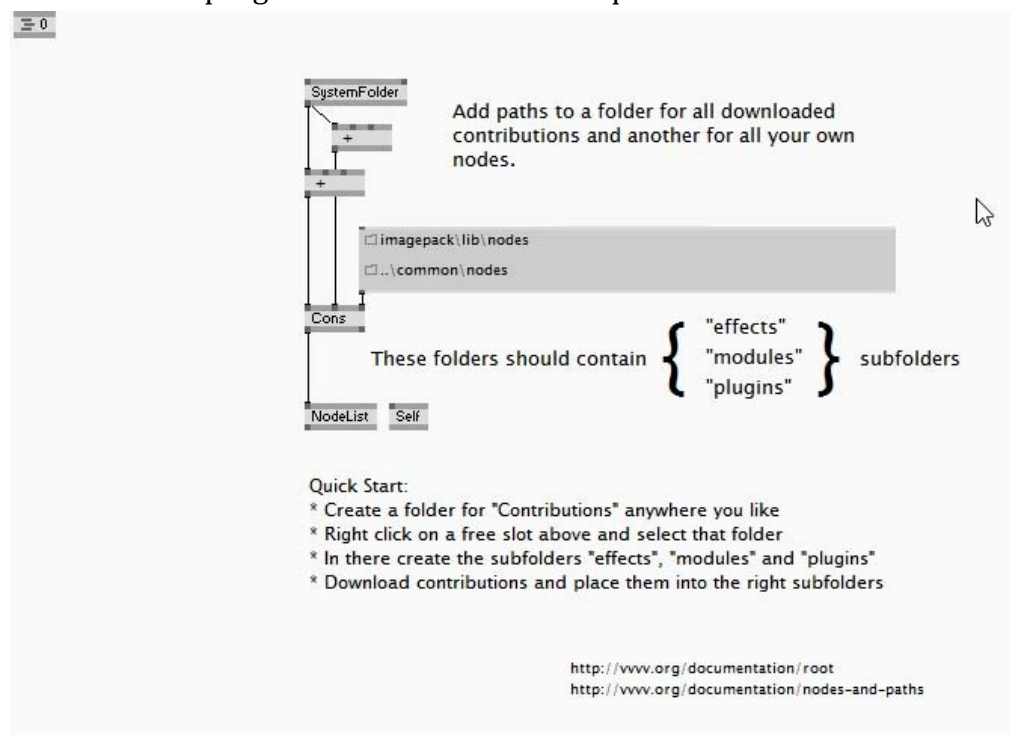
9.13. ábra: Root patch
