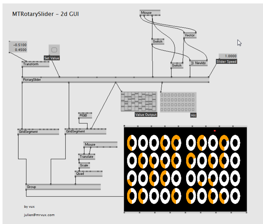
15.8. ábra: Rottary Slider Gui Multitouch
